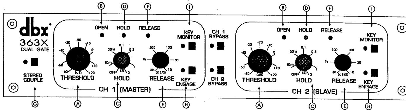
Figure 10: Front Panel
