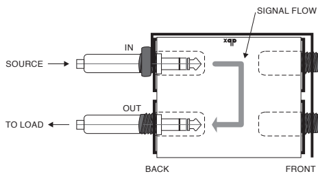
(A) Normalled Patchbay
