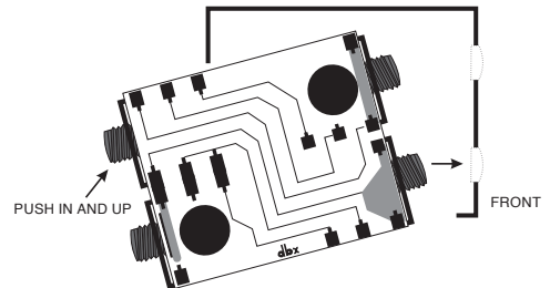
(D) Angle board in (front lower jack to lower front hole), and push rear upper jack (in and up) to snap board into place.
