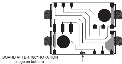
(C) Keeping circuit board component side facing you, rotate the board 180°.
