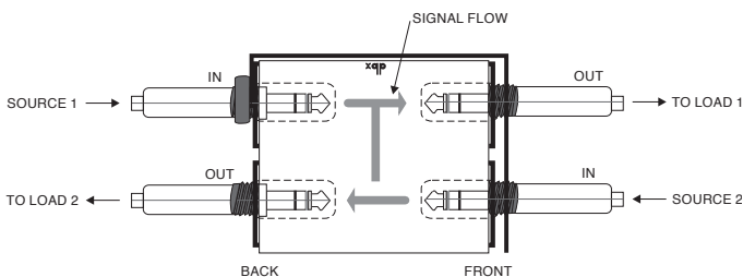
(C) Half-Normalled Patchbay [With Rear-Panel Normal Connection Broken]
