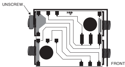
(A) Unscrew rear panel nut and save it.
