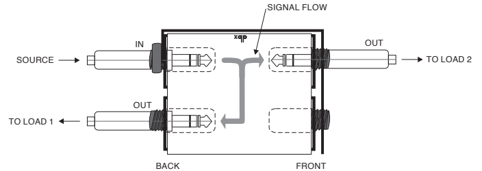
(B) Half-Normalled [Multi-ed] Patchbay
