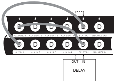
(A) Patching An Effects Device To A Mixer Aux Channel
