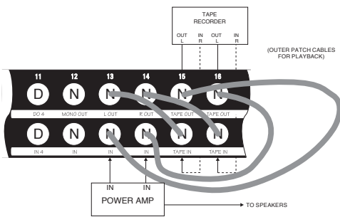
(C) Patching a Tape Recorder To The Main Outs
